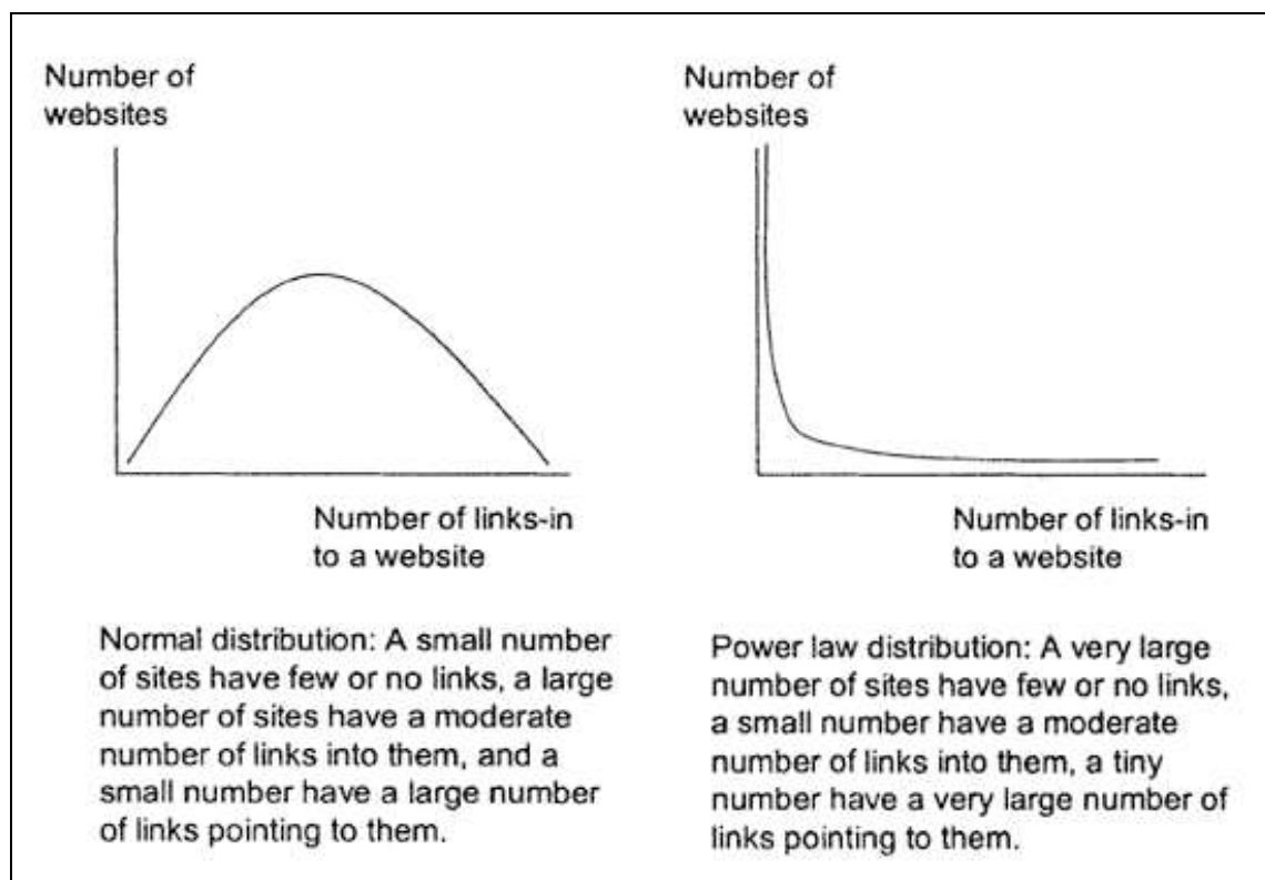
Figure 7.4: Illustration of How Normal Distribution and Power Law Distribution Would Differ in Describing How Many Web Sites Have Few or Many Links Pointing at Them
