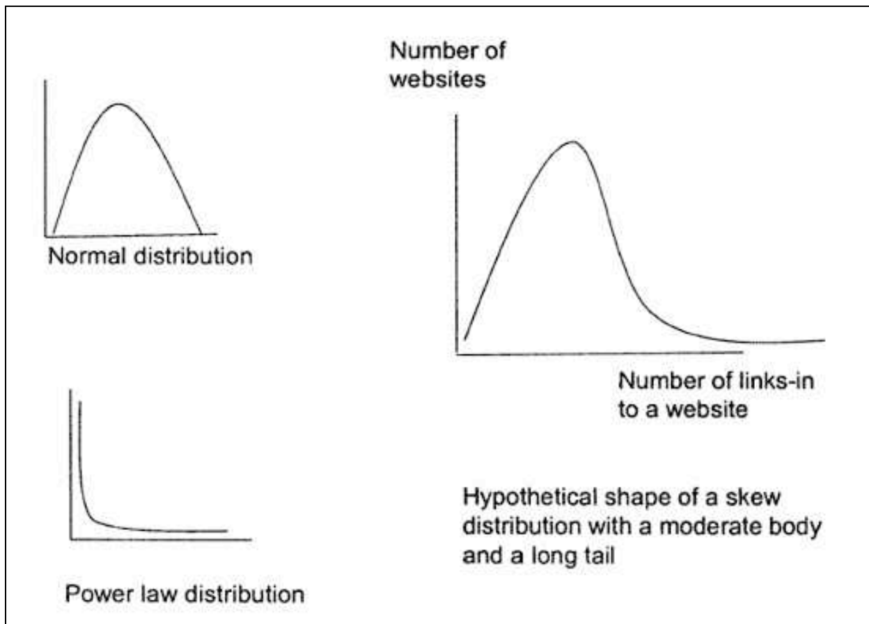
Figure 7.6: Illustration of a Skew Distribution That Does Not Follow a Power Law
